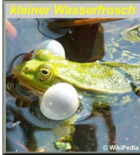
Frosch 2
